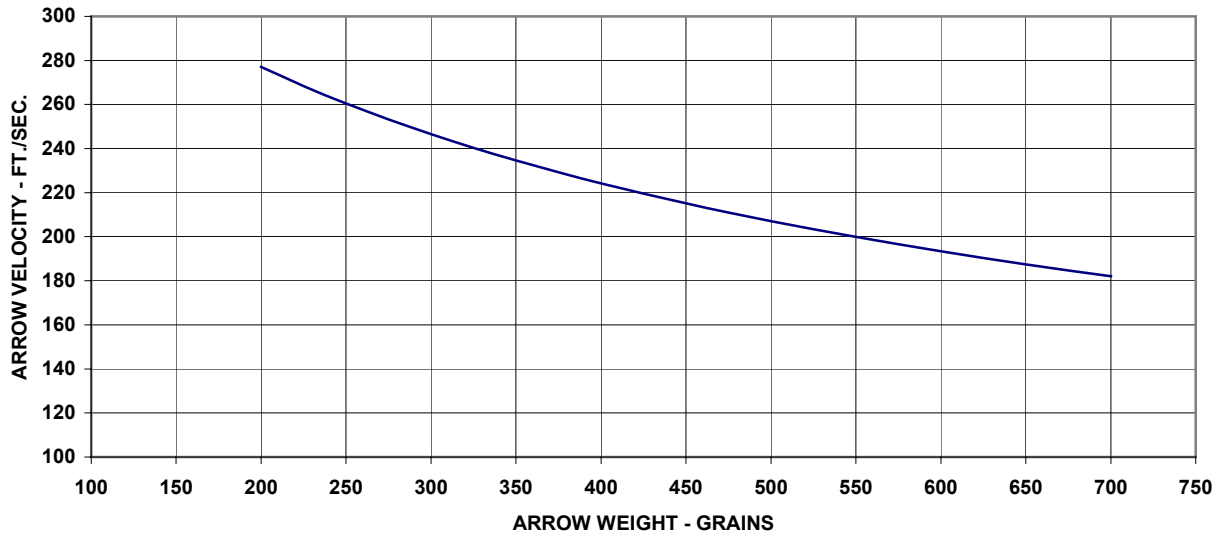
ARROW VELOCITY VS ARROW WEIGHT
