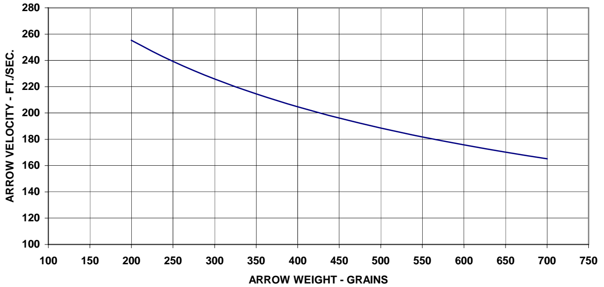
ARROW VELOCITY VS ARROW WEIGHT
