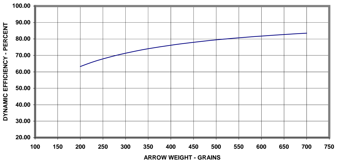
DYNAMIC EFFICIENCY VS ARROW WEIGHT
