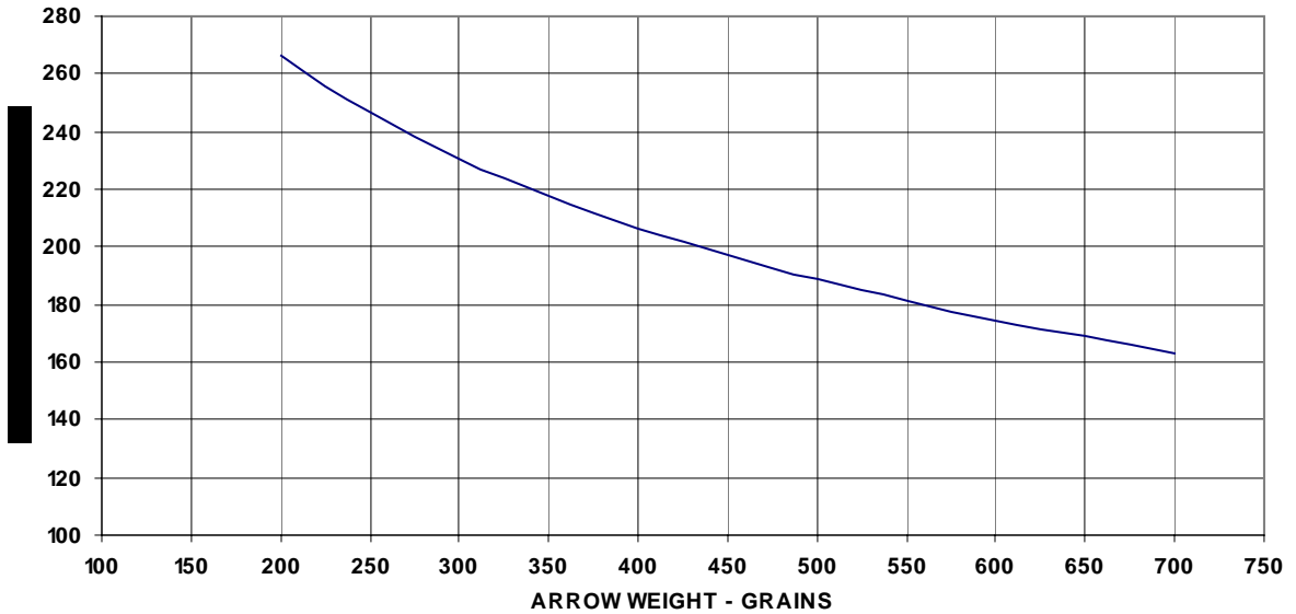
ARROW VELOCITY VS ARROW WEIGHT
