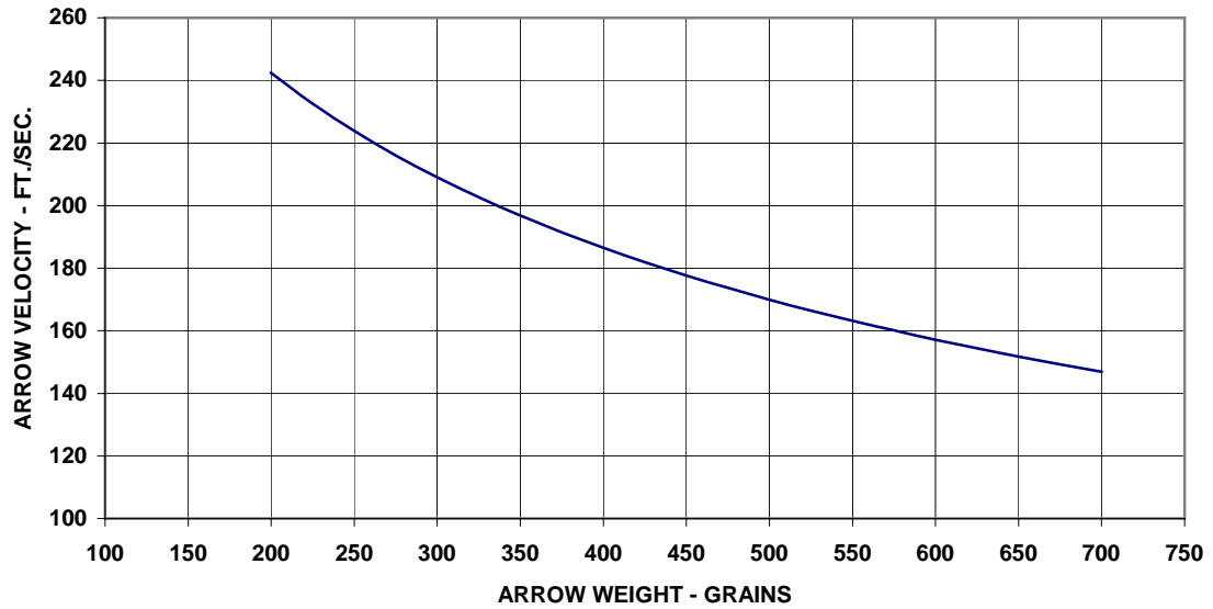
ARROW VELOCITY VS ARROW WEIGHT
