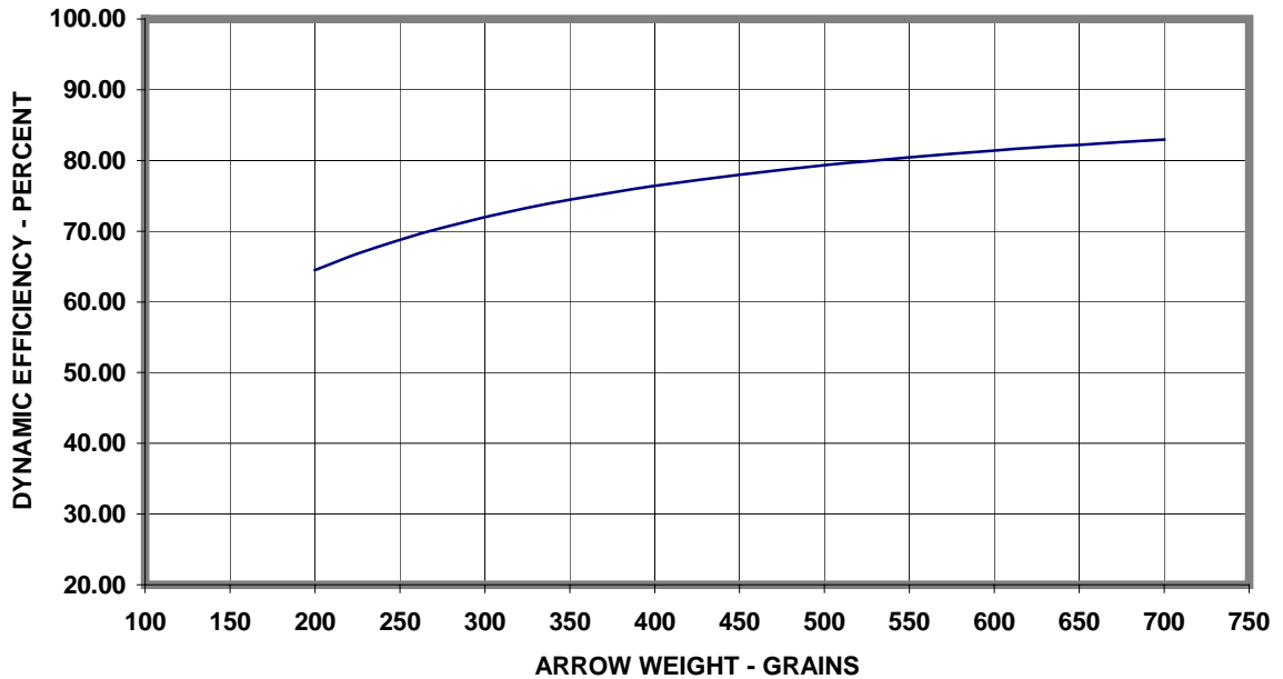
DYNAMIC EFFICIENCY VS ARROW WEIGHT
