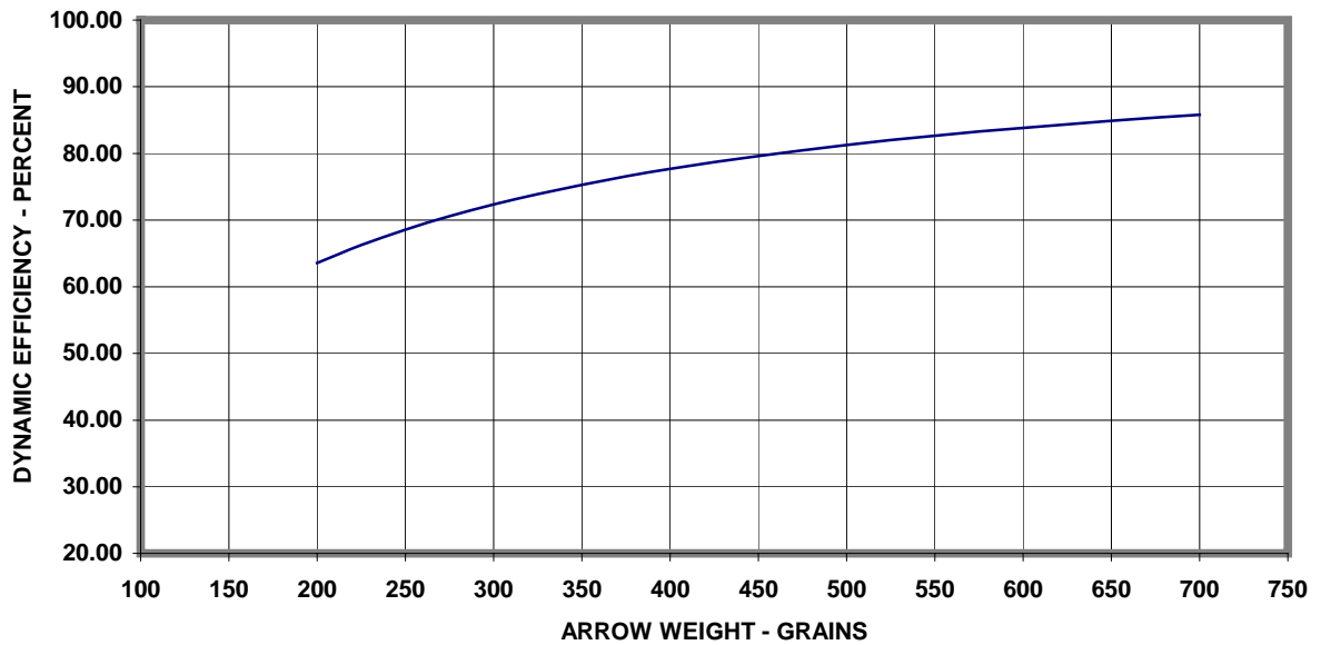
DYNAMIC EFFICIENCY VS ARROW WEIGHT
